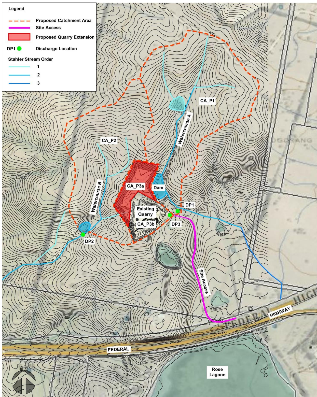
Figure 6 - Proposed Site Catchments and Drainage
