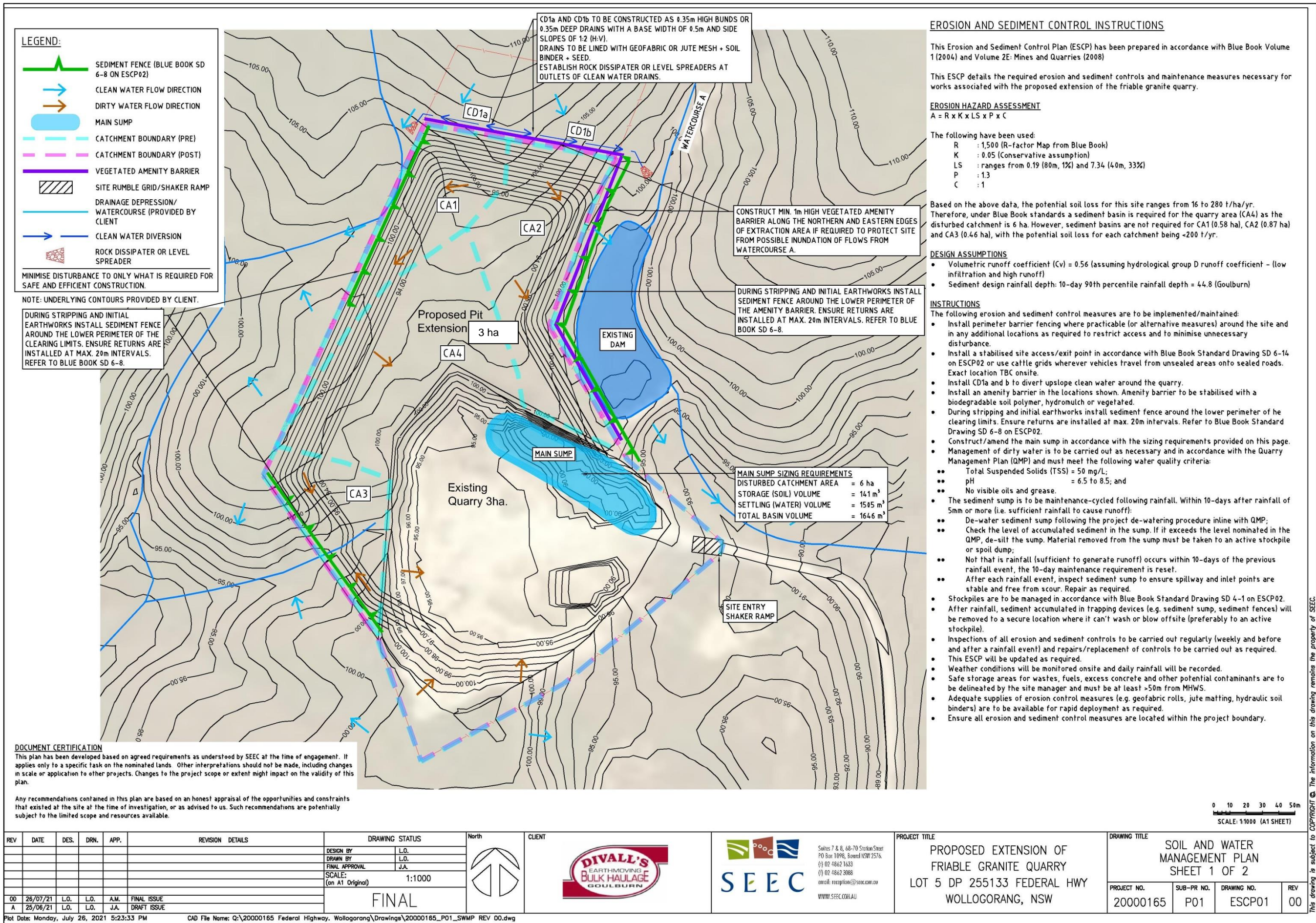
Figure 10 – Location of recommended water management and erosion and sediment control structures
